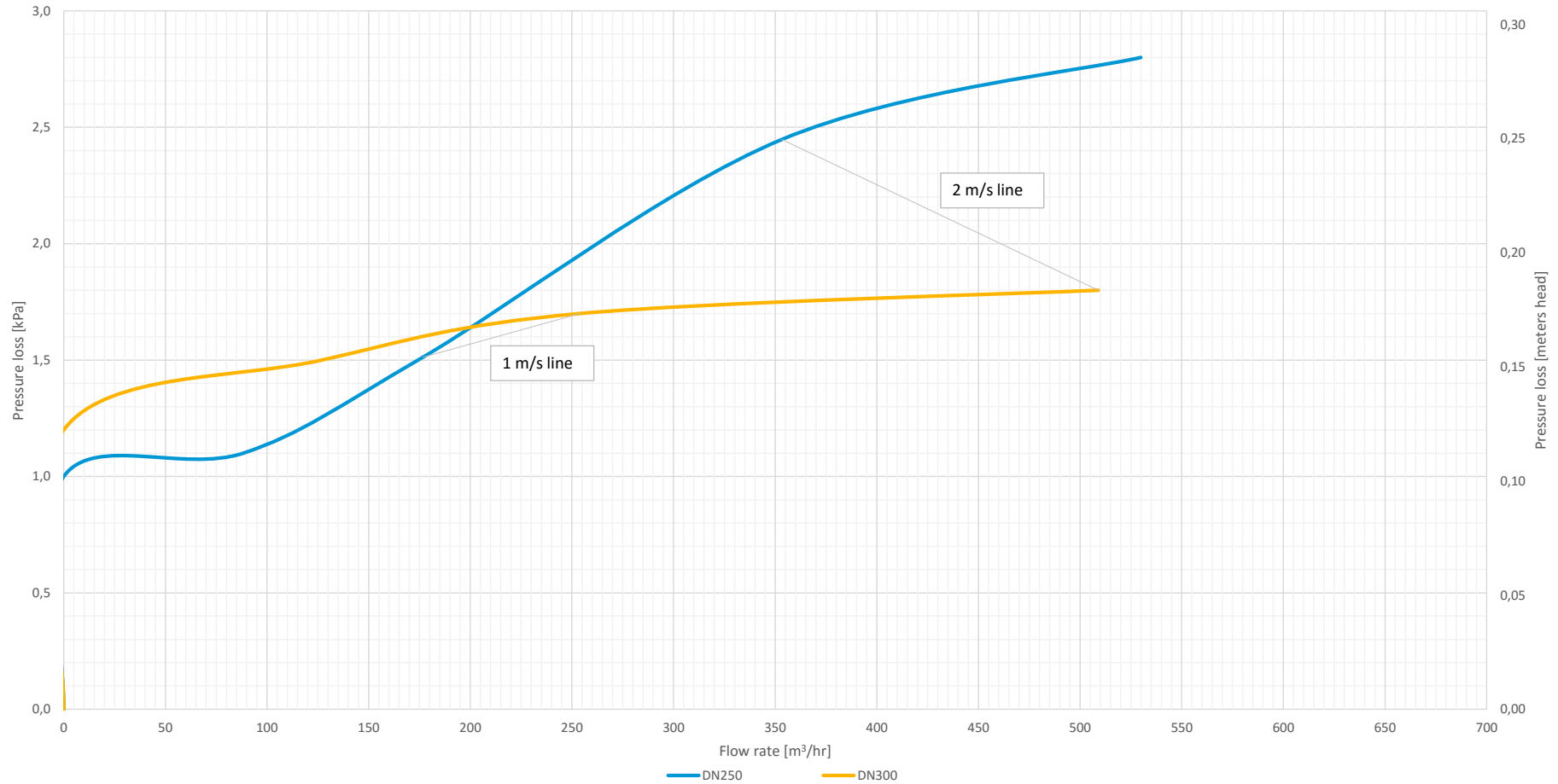
Pressure loss - Series 41 - Spring - DN250 and DN300
