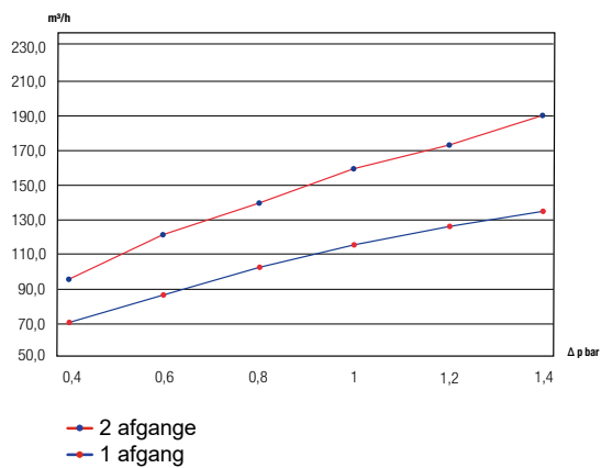
DN80 - 1xB
