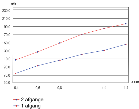
DN80 - 2xB
