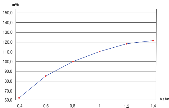
DN80 - 2xB
