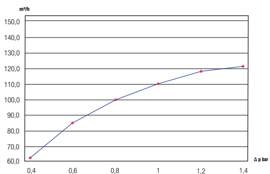
DN80 - 2xB
