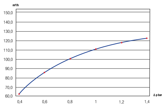
DN80 - 1xB
